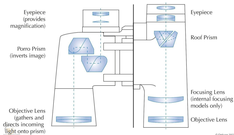
Porro vs Roof Prism designs.
